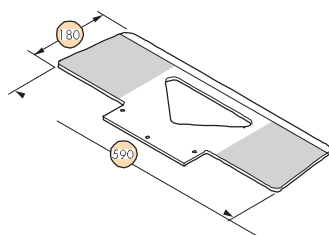
⑨ Art.-Nr. E/1543.930074 Schaufel XWL
