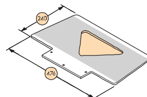
④ Art.-Nr. E/1543.930030 Schaufel GS
