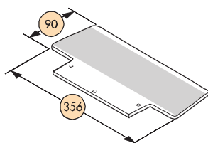
⑥ Art.-Nr. E/1543.930008 Schaufel W
